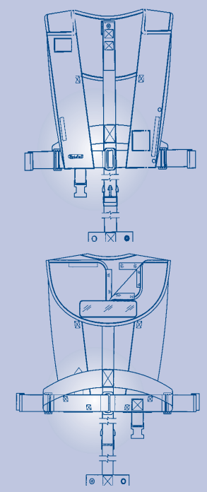
MK28WB General Assembly
